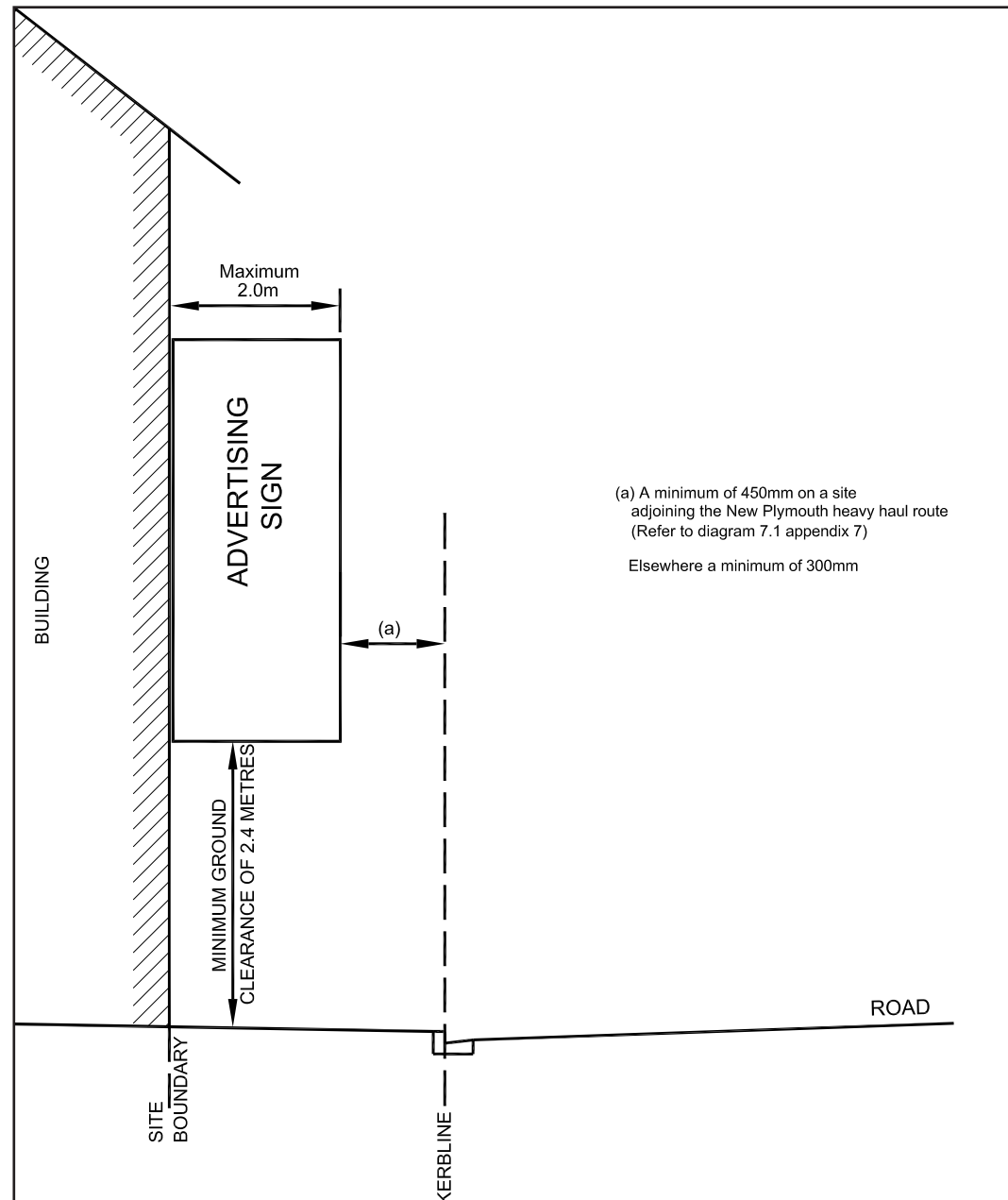
Diagram 1.1 Maximum projection of an ADVERTISING SIGN over the ROAD BOUNDARY within all BUSINESS ENVIRONMENT AREAS
